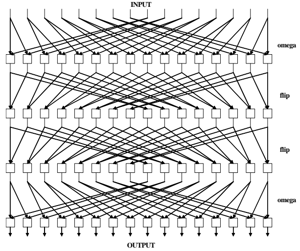
Figure 2. A 16-bit omega-flip network
